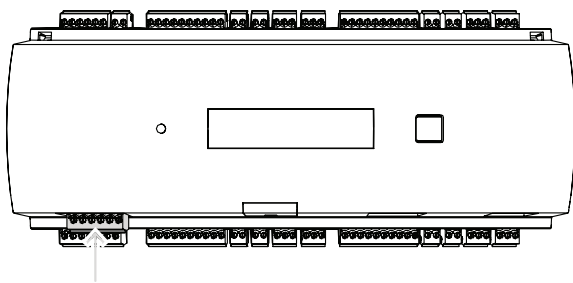
Figure 4.10: interface hôte RS-485
