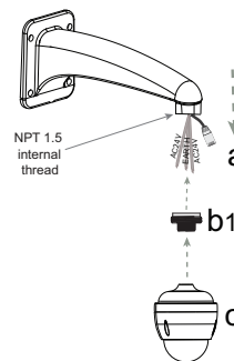
Fig. 1: Example installation: AUTODOME IP 4000 HD camera + NPT 1.5 to G 3/4 adapter + third-party wall mount
