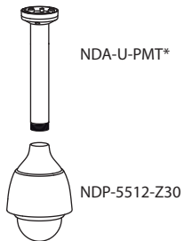
Fig. 2: Pendant Pipe mount * NDA-U-PMTE: optional 50cm / 20" extension pipe
