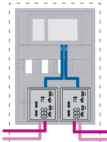
Figura 7.6: Conectar redes Ethernet
