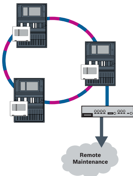
Рис. 8.4: Remote Maintenance
