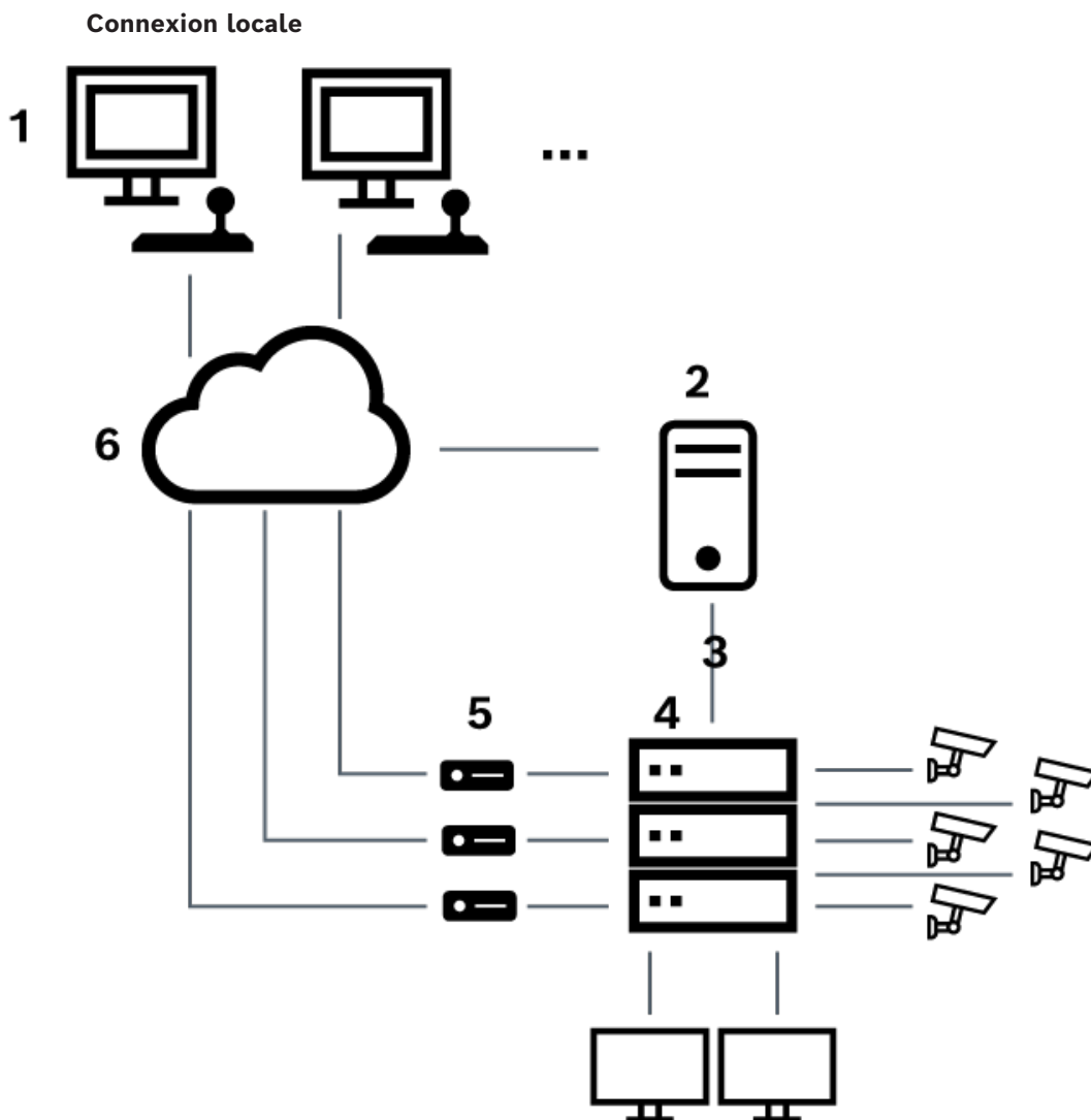
Figure 6.3: Connexion locale de Bosch Video Management System à la matrice Allegiant Bosch
