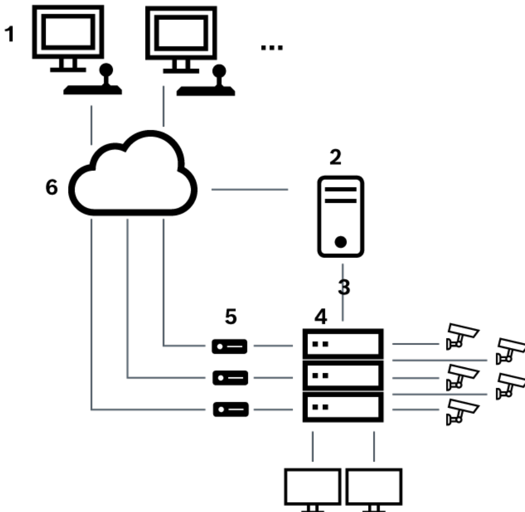
Figure 6.3: Connexion locale de Bosch Video Management System à la matrice Allegiant Bosch
