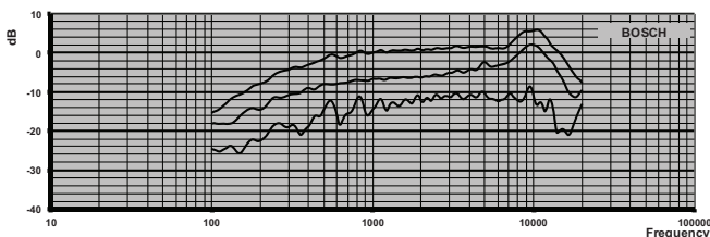
Fig. 1: Frequency response (Opening angle: 0, 90 and 180 degrees)
