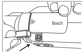
Figure 4.6 Lens connector
