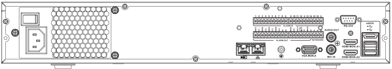
Fig. 1: DIVAR 5000 network back panel (no PoE)
