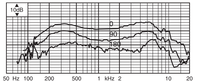
Frequenzgang
