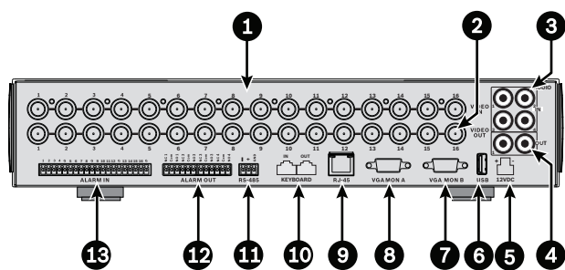
Connections on back of DVR 630/650 (16-channel version)
