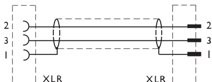
LBC 1208/40 (10 m)
