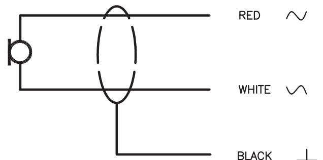
Diagram sirkuit
