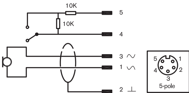
Diagram sirkuit
