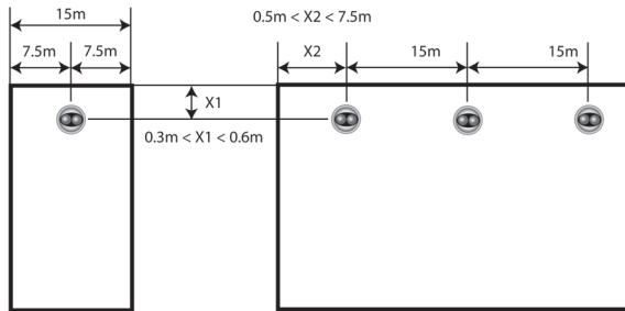
Fig. 2: Mounting (flat ceiling)
