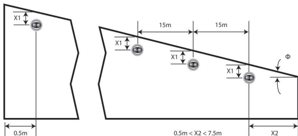
Fig. 3: Mounting (shed roof)
