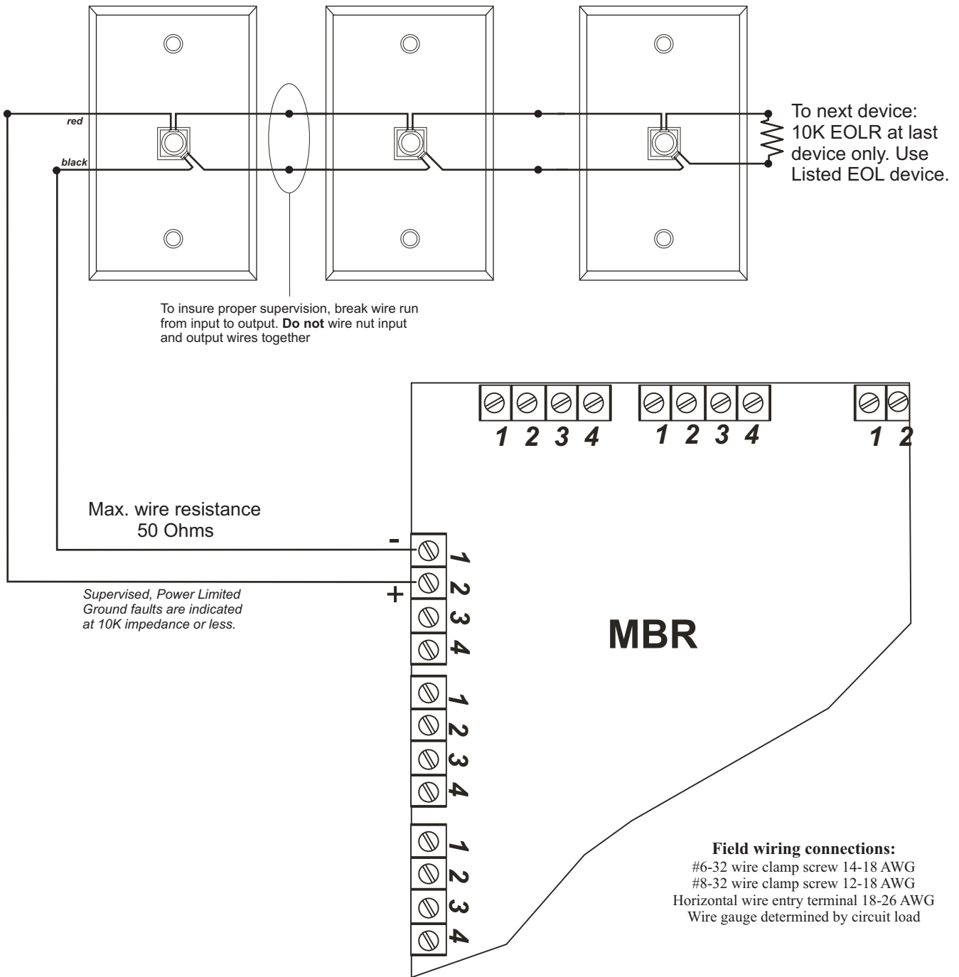
Fig 3 Sample Connection Details
