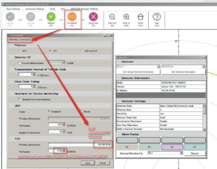
Configure the OPTEX detectors to send information to the BVMS.
