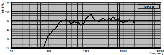
Frequenzgang
