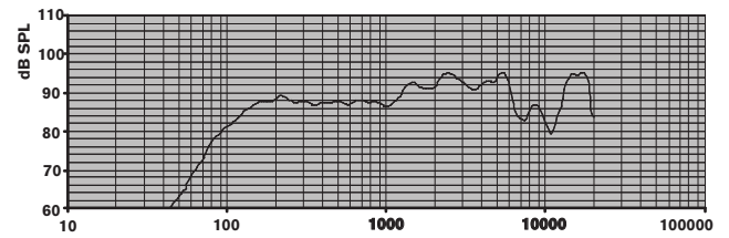
Fig. 11: LC1-WC06E8_Frequency response
