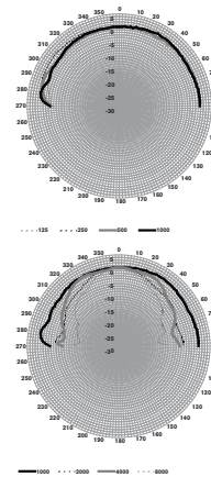
Fig. 16: LC1-WM06E8 Polar diagrams
