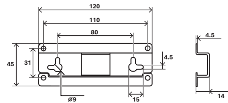
Fig. 2: Bracket dimensions
