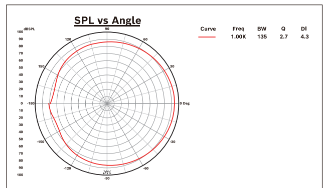
Fig. 5: Polar pattern diagram: 1K horizontal directivity
