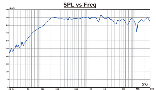
Fig. 3: Frequency response graph
