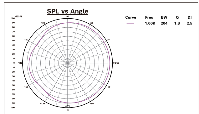
Fig. 4: Polar pattern diagram: 1K vertical directivity
