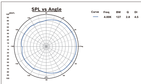
Fig. 7: Polar pattern diagram: 4K horizontal directivity
