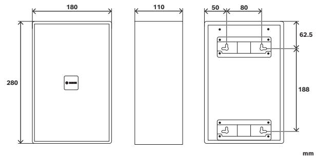
Fig. 1: Front, side and rear view
