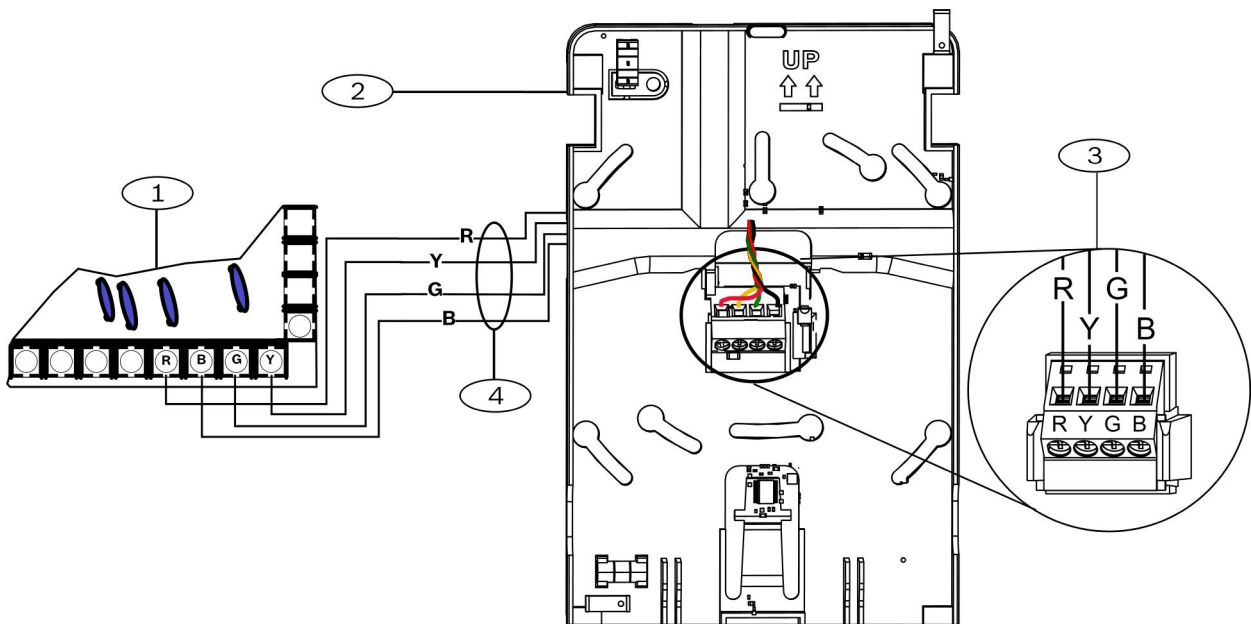
Figure 3.4: Wiring to an Option Bus Terminal Strip
