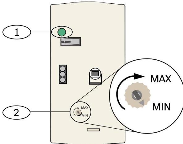
Figure 6.8: Sensitivity settings
