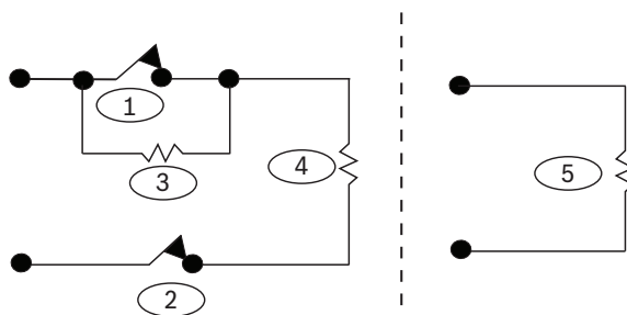
Figure 12.12: Dual EOL resistor option
