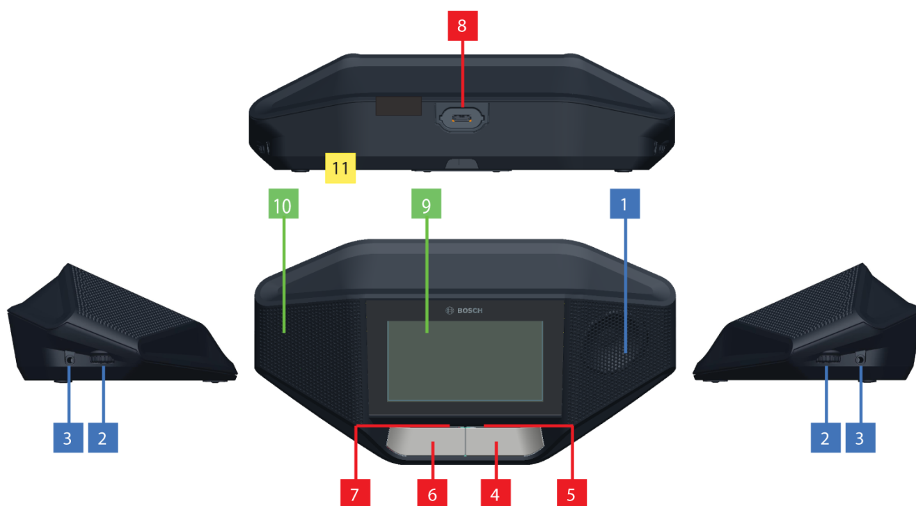
Figura 3.1: DCNM-DE
